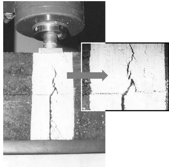
Figure 4 – Crack propagation without geogrid
