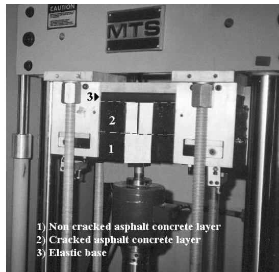
Figure 2 – Fatigue Test with MTS equipment.
