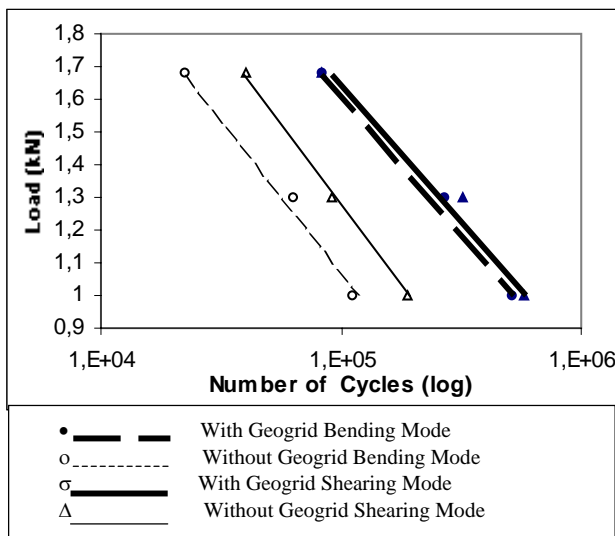
Figure 8 – Fatigue curves.
