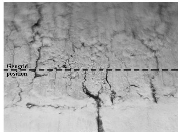
Figure 5 – Beam with geogrid in bending mode
